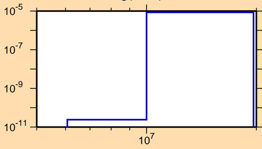
\sigma vs. E for ^{95}\text{Ag}(n,n\alpha)
