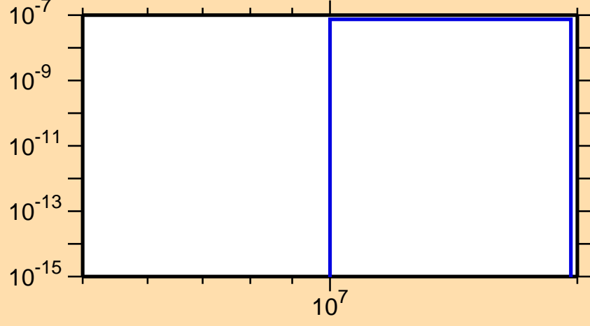
\sigma vs. E for ^{95}\text{Ag} (mt 45)
