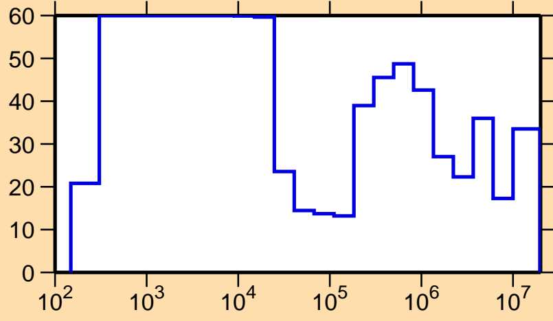
\Delta\sigma/\sigma vs. E for ^{95}\text{Ag}(n,el.)
