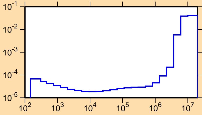
\sigma vs. E for ^{95}\text{Ag}(n,\alpha)
