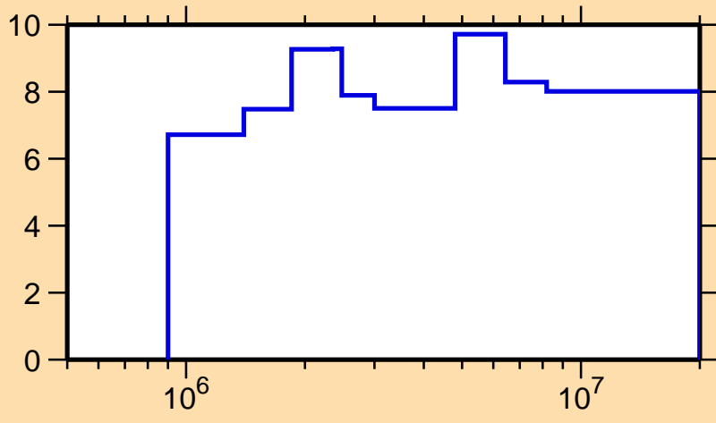
\Delta\sigma/\sigma vs. E for ^{95}\text{Ag}(n,n_{\text{nonel}})
