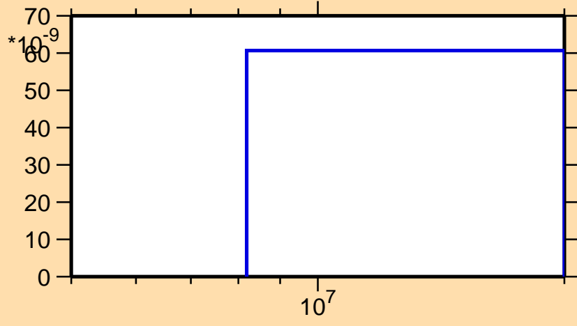
\sigma vs. E for ^{95}\text{Ag} (mt 45)
