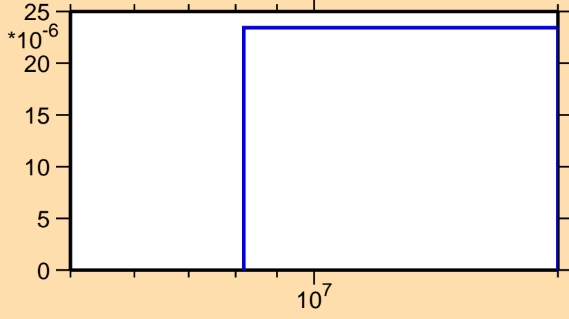
\sigma vs. E for ^{95}\text{Ag}(n,t)
