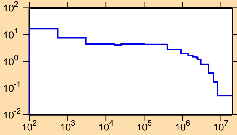
\sigma vs. E for ^{95}\text{Ag}(n,p)
