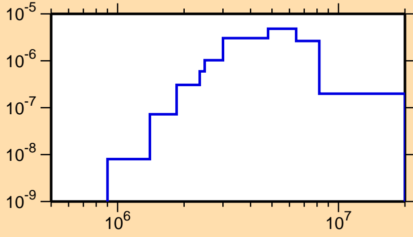
\sigma vs. E for ^{96}\text{Ag}(n,n_2)
