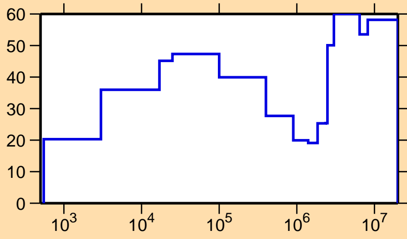
\Delta\sigma/\sigma vs. E for ^{96}\text{Ag}(n,p)
