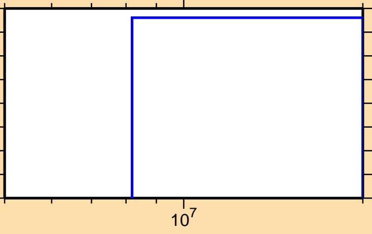
\sigma vs. E for ^{96}\text{Ag} (mt 34)
