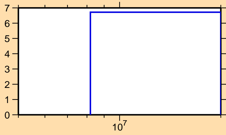
\Delta\sigma/\sigma vs. E for ^{96}\text{Ag}(n,\text{el.})
