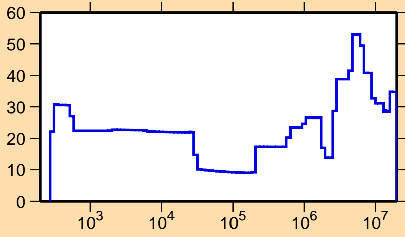
\Delta\sigma/\sigma vs. E for ^{96}\text{Ag}(n,el.)
