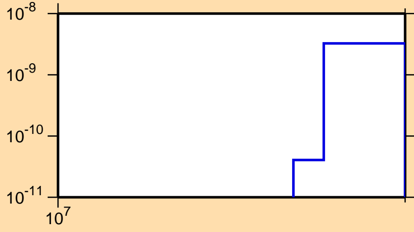
\sigma vs. E for ^{96}\text{Ag} (mt 34)
