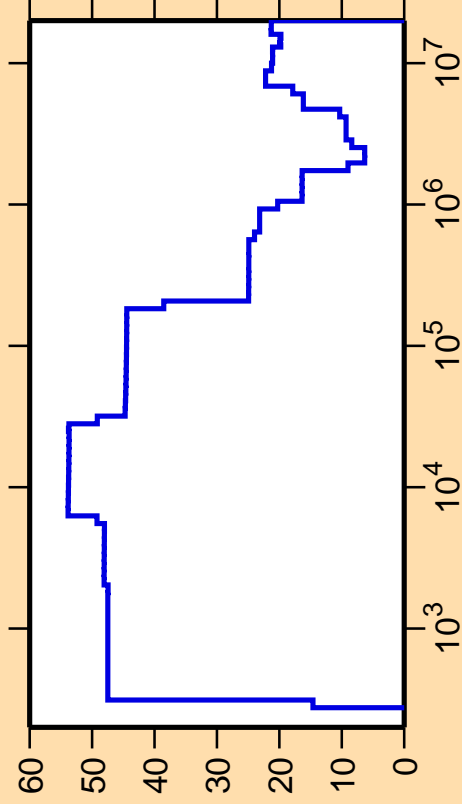
\Delta\sigma/\sigma vs. E for ^{96}\text{Ag}(n,\text{nonel.})
