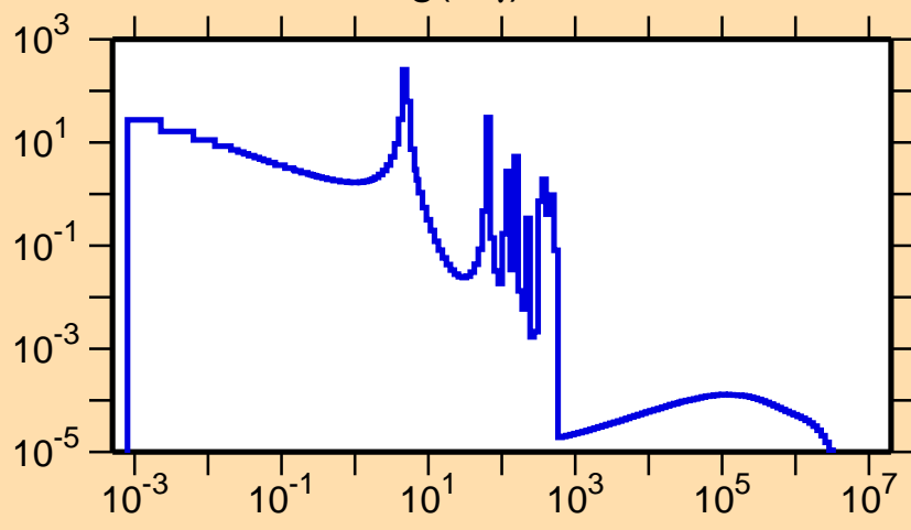
\sigma vs. E for ^{96}\text{Ag}(n,\gamma)
