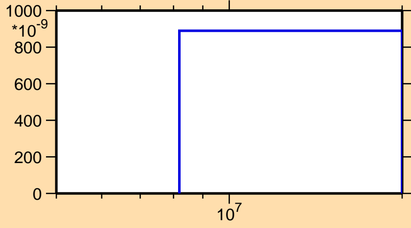
\sigma vs. E for ^{96}\text{Ag}(n,pt)
