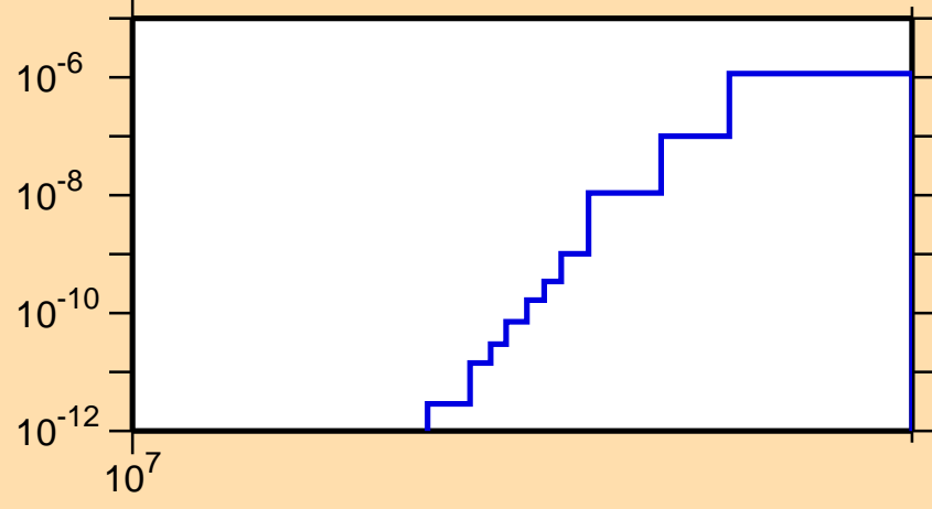
\sigma vs. E for ^{97}\text{Ag} (mt 45)
