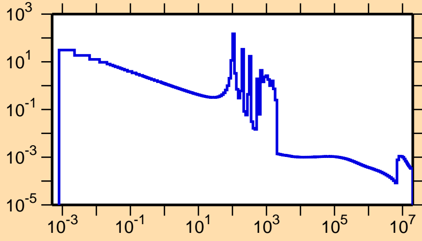
\sigma vs. E for ^{97}\text{Ag}(n,\gamma)
