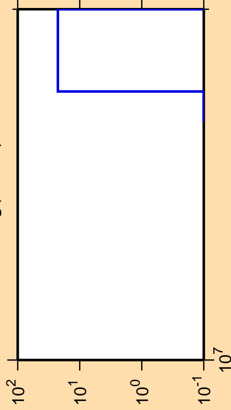
\Delta\sigma/\sigma vs. E for ^{97}\text{Ag} (mt 34)
