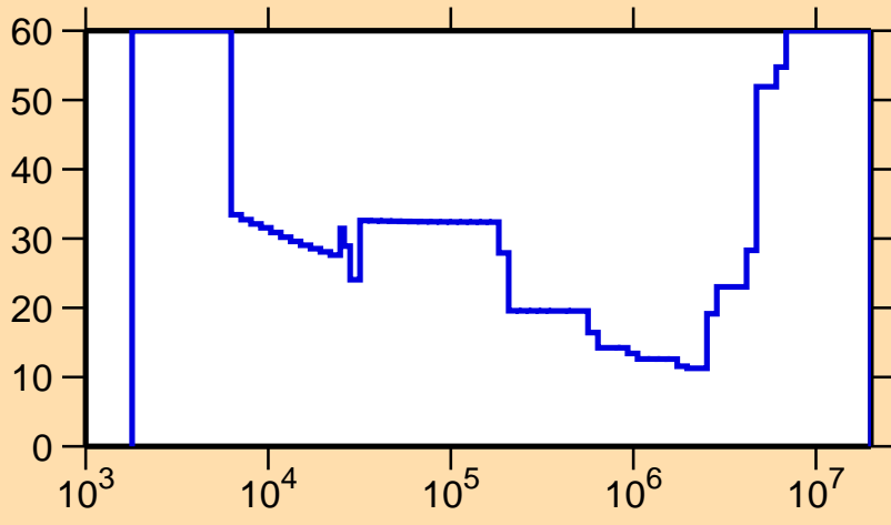
\Delta\sigma/\sigma vs. E for ^{97}\text{Ag}(n,p)
