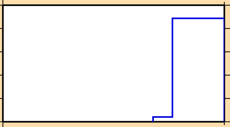
\sigma vs. E for ^{97}\text{Ag} (mt 34)
