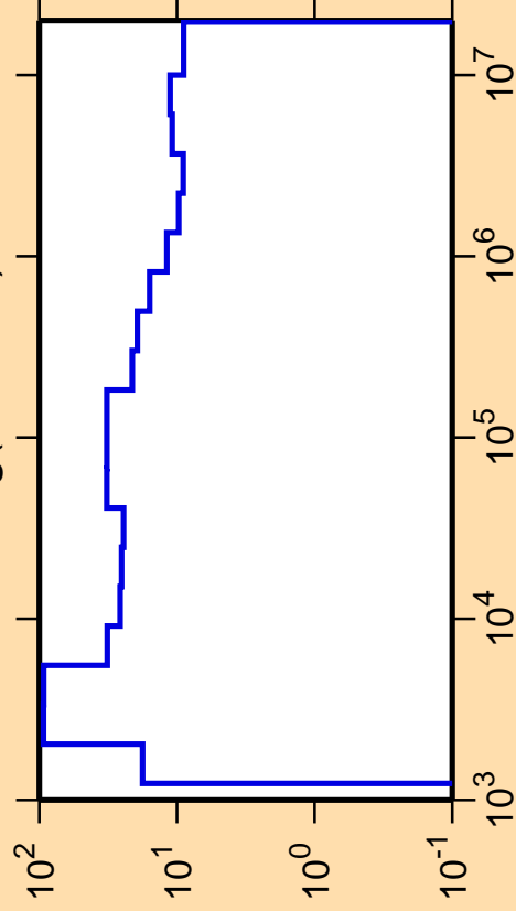
\Delta\sigma/\sigma vs. E for ^{97}\text{Ag}(n,\text{nonel.})
