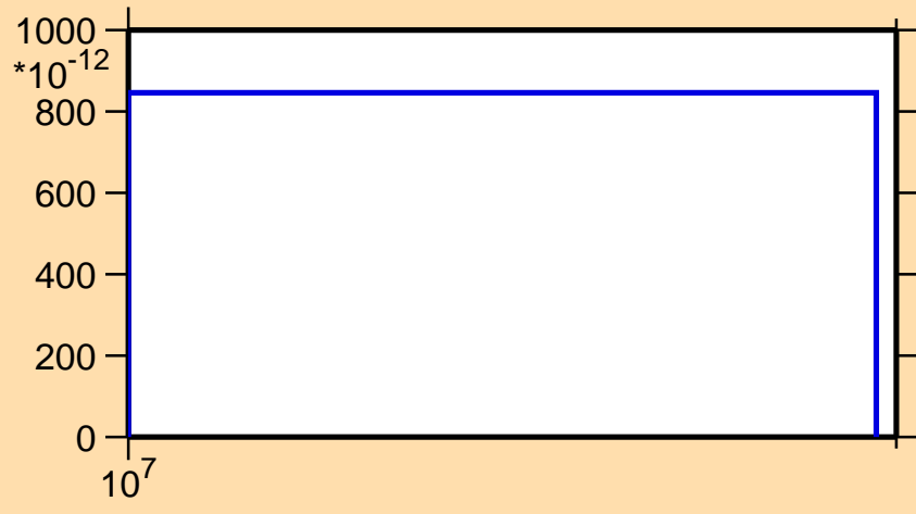
\sigma vs. E for ^{97}\text{Ag}(n,\text{pt})
