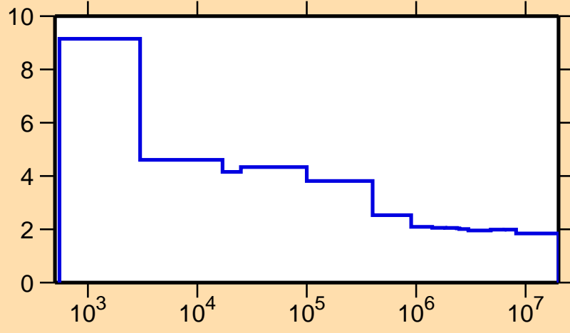
\sigma vs. E for ^{97}\text{Ag}(n,\text{nonel.})
