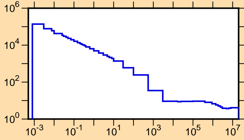
\sigma vs. E for ^{97}\text{Ag}(n,\text{tot.})
