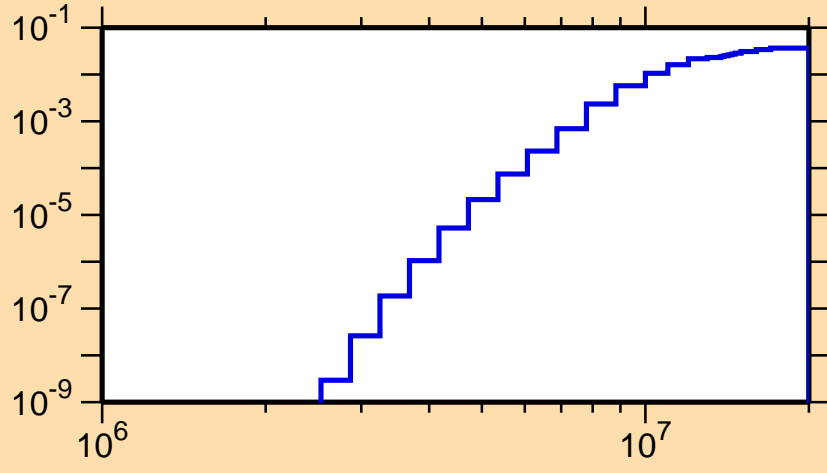
\sigma vs. E for ^{98}\text{Ag}(n,d)
