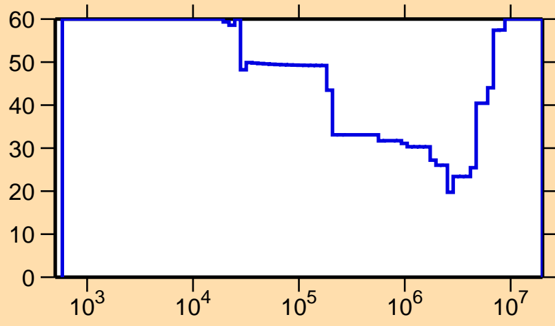
\Delta\sigma/\sigma vs. E for ^{98}\text{Ag}(n,p)
