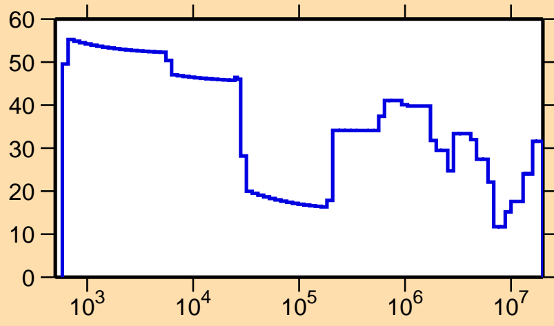
\Delta\sigma/\sigma vs. E for ^{98}\text{Ag}(n,\text{el.})
