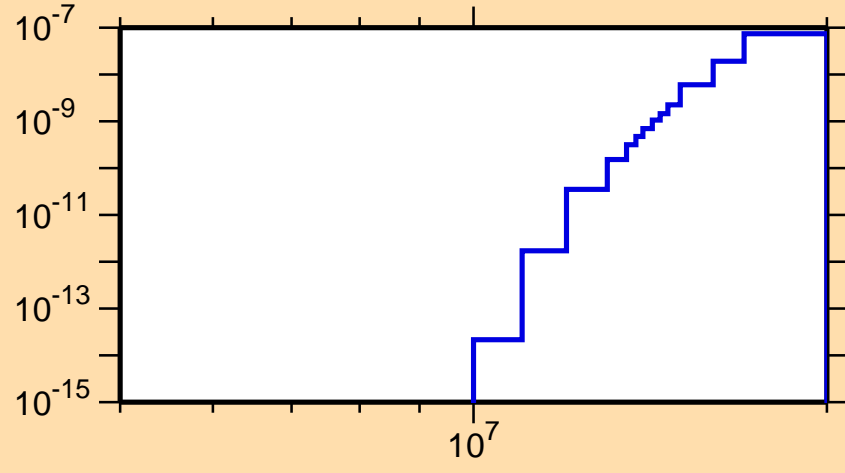
\sigma vs. E for ^{98}\text{Ag}(\text{mt117})
