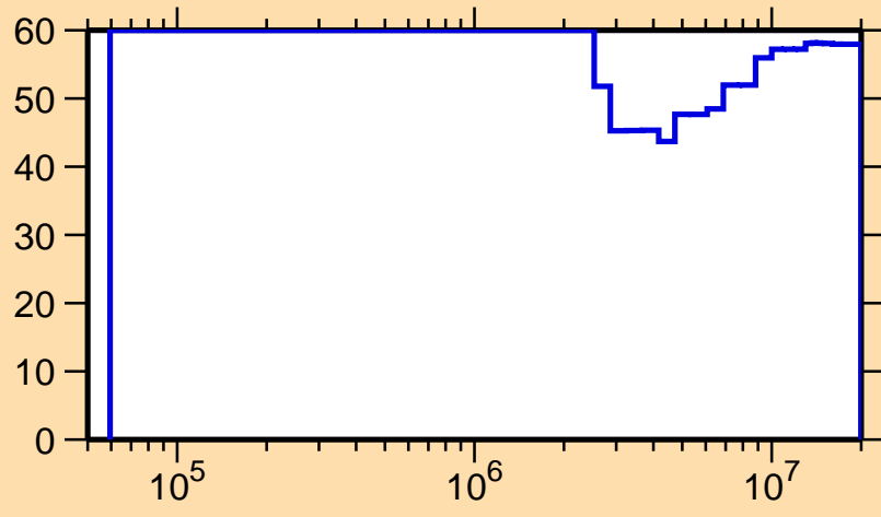
\Delta\sigma/\sigma vs. E for ^{98}\text{Ag}(n,\text{inel.})
