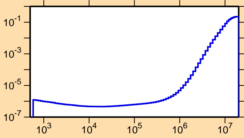
\sigma vs. E for ^{98}\text{Ag}(n,p\alpha)
