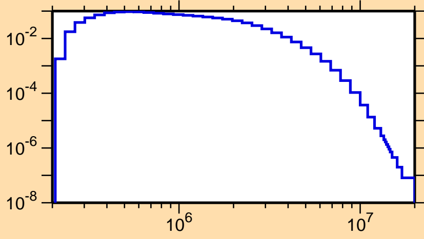
\sigma vs. E for ^{98}\text{Ag}(n,n_3)
