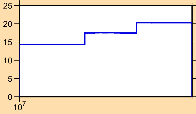
\Delta\sigma/\sigma vs. E for ^{98}\text{Ag}(n,\text{tot.})
