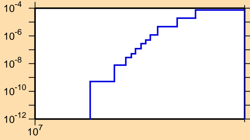
\sigma vs. E for ^{98}\text{Ag}(n,\text{nd})
