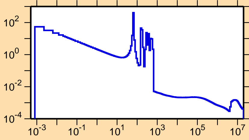
\sigma vs. E for ^{98}\text{Ag}(n,\gamma)
