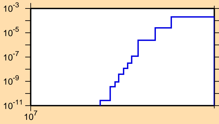
\sigma vs. E for ^{98}\text{Ag}(n,\text{pt})
