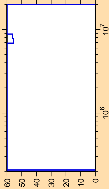
\Delta\sigma/\sigma vs. E for ^{98}\text{Ag}(n,n_3)
