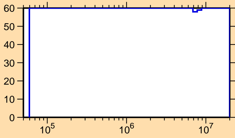
\Delta\sigma/\sigma vs. E for ^{98}\text{Ag}(n,n_1)
