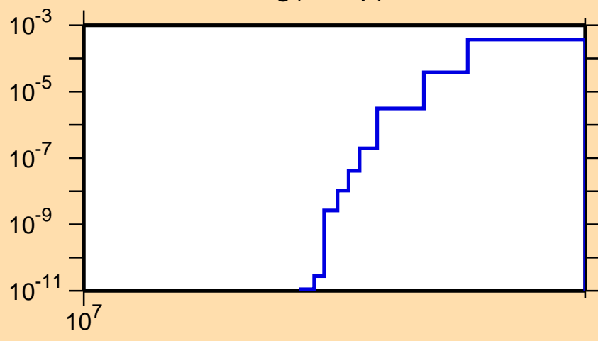
\sigma vs. E for ^{98}\text{Ag}(n,2np)
