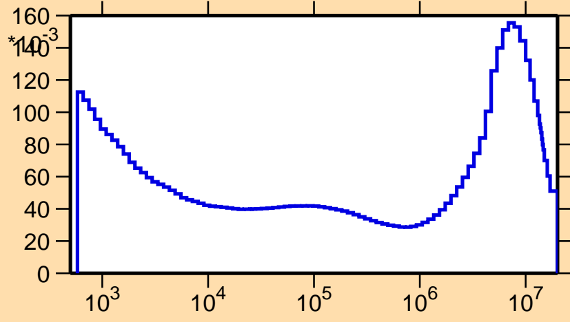
\sigma vs. E for ^{98}\text{Ag}(n,\alpha)
