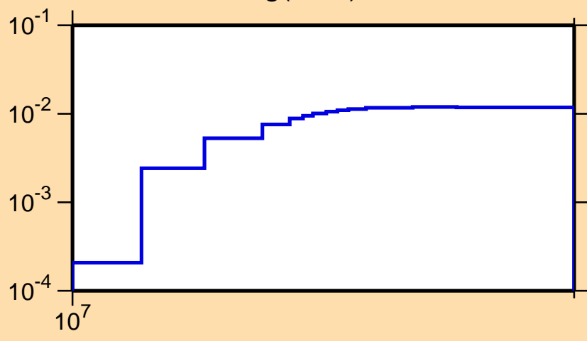
\sigma vs. E for ^{98}\text{Ag}(n,2n)
