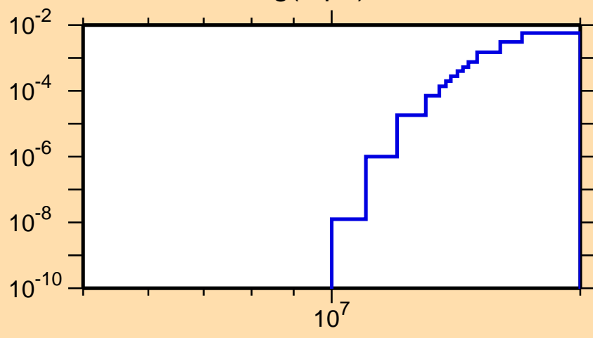
\sigma vs. E for ^{98}\text{Ag}(n,\text{pd})
