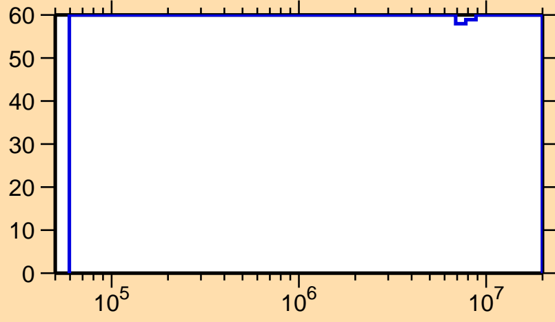
\Delta\sigma/\sigma vs. E for ^{98}\text{Ag}(n,n_1)
