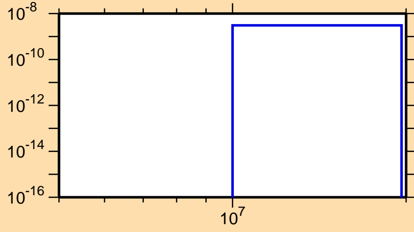
\sigma vs. E for ^{98}\text{Ag}(\text{mt117})
