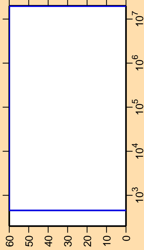
\Delta\sigma/\sigma vs. E for ^{98}\text{Ag}(n,p\alpha)
