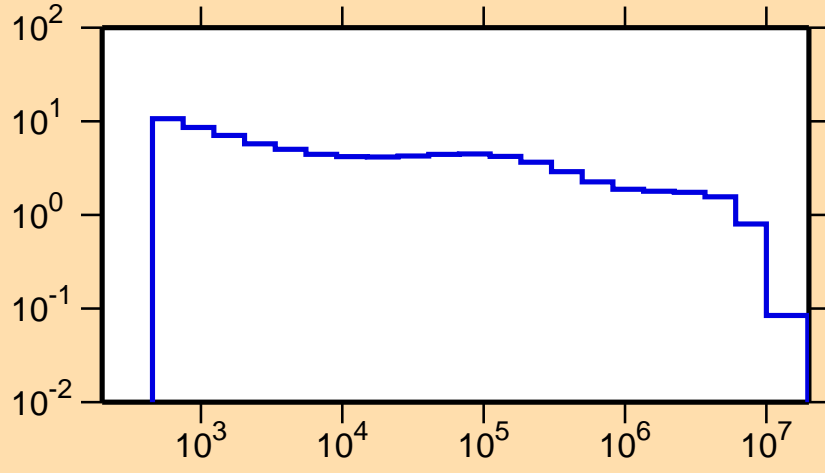
\sigma vs. E for ^{98}\text{Ag}(n,p)
