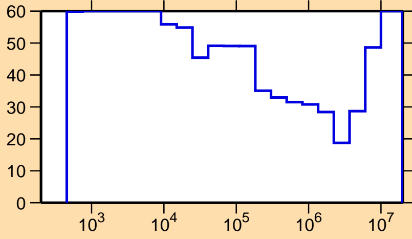
\Delta\sigma/\sigma vs. E for ^{98}\text{Ag}(n,p)
