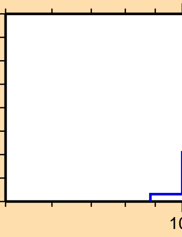
\sigma vs. E for ^{99}\text{Ag}(\text{mt117})
