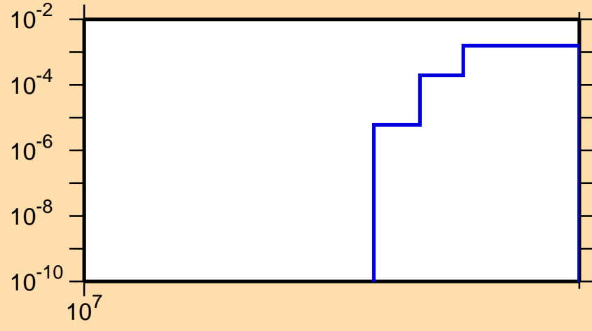
\sigma vs. E for ^{99}\text{Ag}(n,2np)
