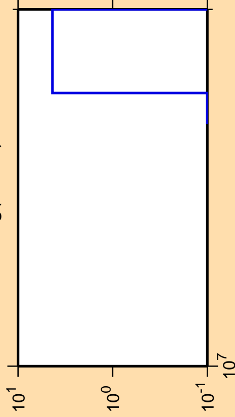
\Delta\sigma/\sigma vs. E for ^{99}\text{Ag}(n,2n\alpha)
