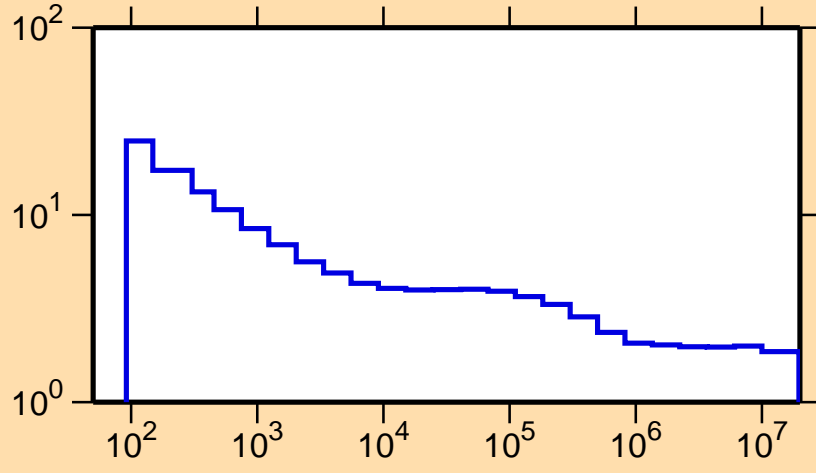
\sigma vs. E for ^{100}\text{Ag}(n,\text{nonel.})
