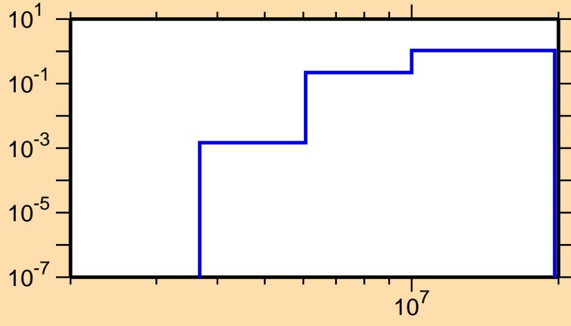
\sigma vs. E for ^{100}\text{Ag}(n,np)
