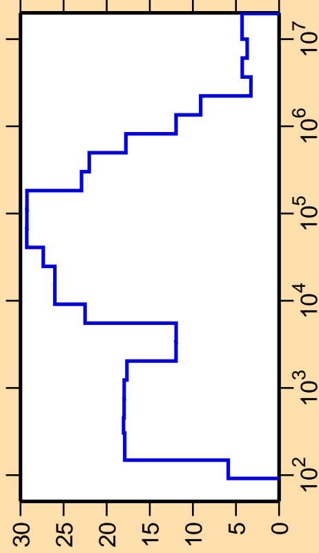
\Delta\sigma/\sigma vs. E for ^{100}\text{Ag}(n,\text{nonel.})
