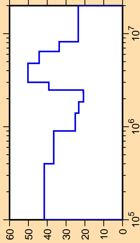
\Delta\sigma/\sigma vs. E for ^{100}\text{Ag}(n,n_4)
