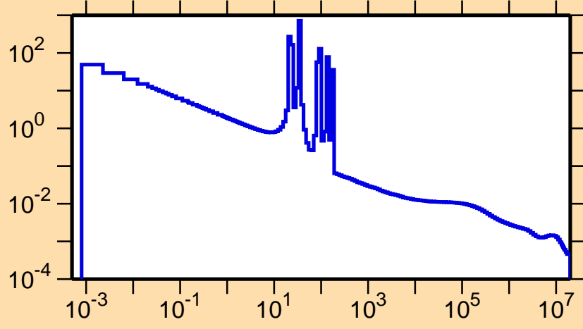
\sigma vs. E for ^{100}\text{Ag}(n,\gamma)
