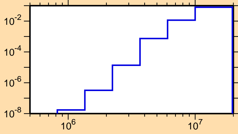
\sigma vs. E for ^{100}\text{Ag}(n,p\alpha)
