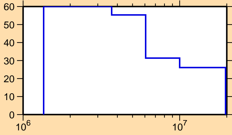
\Delta\sigma/\sigma vs. E for ^{100}\text{Ag}(n,n\text{cont.})
