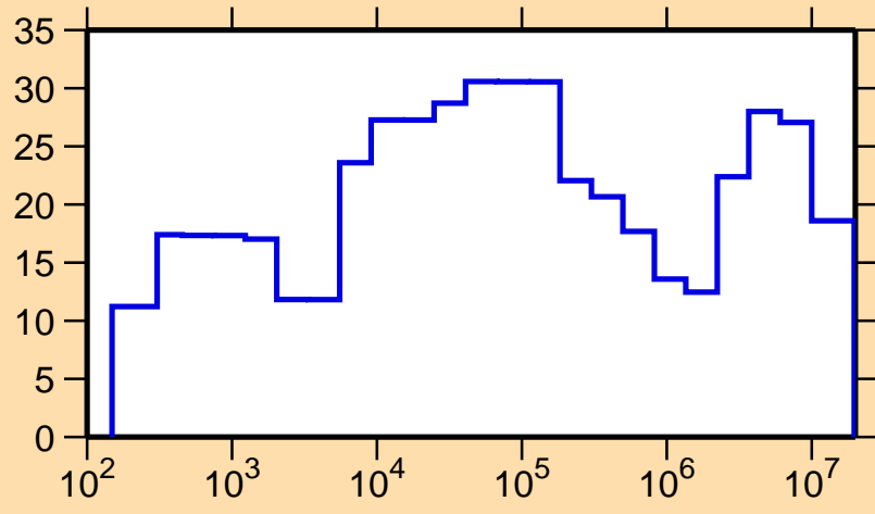
\Delta\sigma/\sigma vs. E for ^{100}\text{Ag}(n,p)
