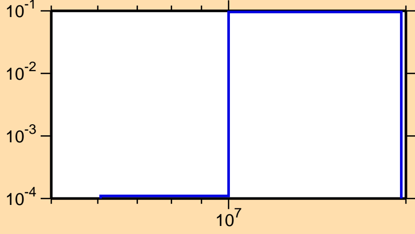
\sigma vs. E for ^{100}\text{Ag}(n,2n)
