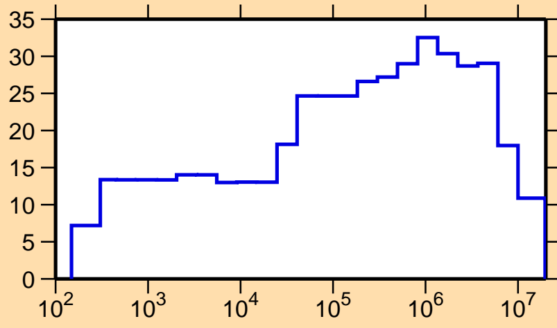
\Delta\sigma/\sigma vs. E for ^{101}\text{Ag}(n,p)
