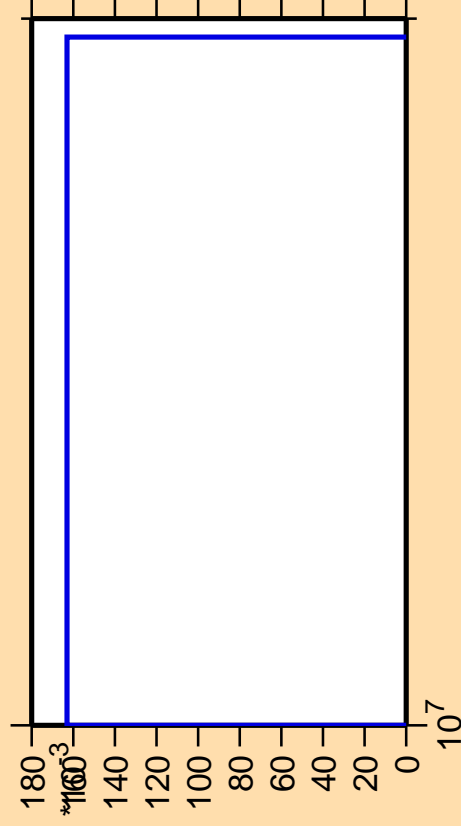
\Delta\sigma/\sigma vs. E for ^{101}\text{Ag} (mt 34)
