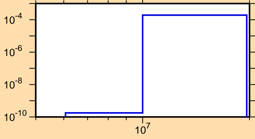
\sigma vs. E for ^{101}\text{Ag}(n,t)
