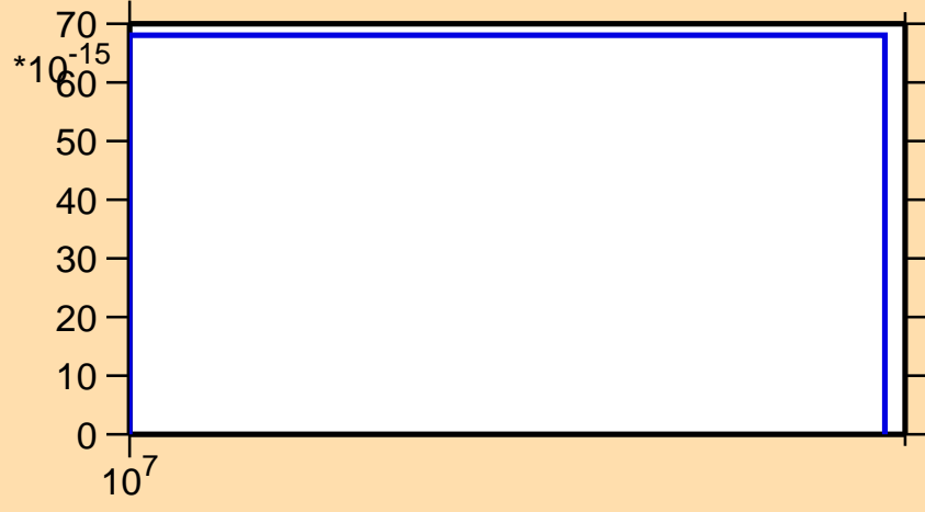
\sigma vs. E for ^{101}\text{Ag} (mt 34)
