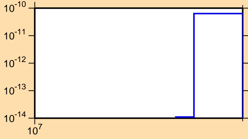
\sigma vs. E for ^{101}\text{Ag}(\text{mt } 34)
