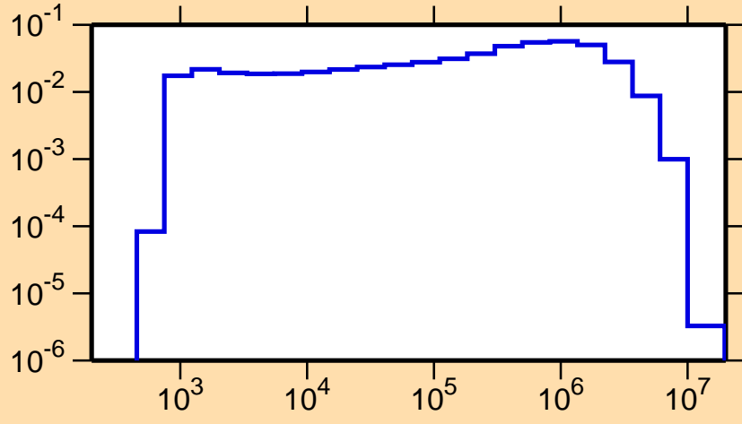
\sigma vs. E for ^{101}\text{Ag}(n,n_1)
