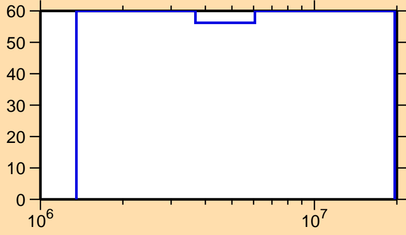
\Delta\sigma/\sigma vs. E for ^{101}\text{Ag}(n,n\text{cont.})
