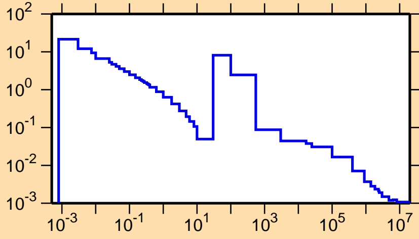
\sigma vs. E for ^{101}\text{Ag}(n,\gamma)
