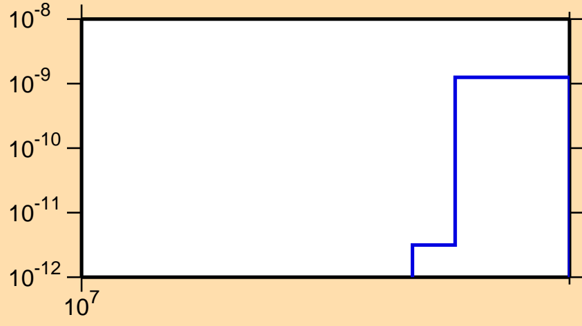
\sigma vs. E for ^{102}\text{Ag} (mt 34)
