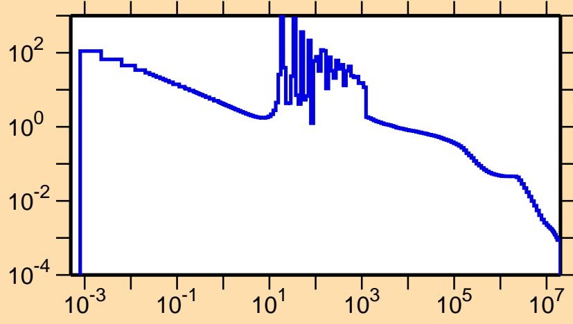
\sigma vs. E for ^{102}\text{Ag}(n,\gamma)
