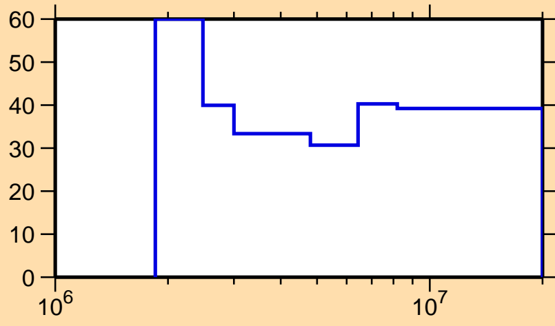
\Delta\sigma/\sigma vs. E for ^{102}\text{Ag}(n,n\text{cont.})
