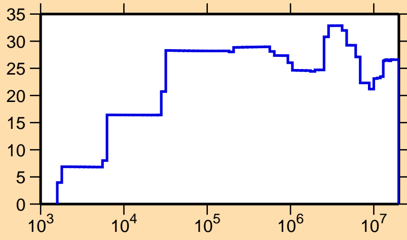
\Delta\sigma/\sigma vs. E for ^{102}\text{Ag}(n,p)
