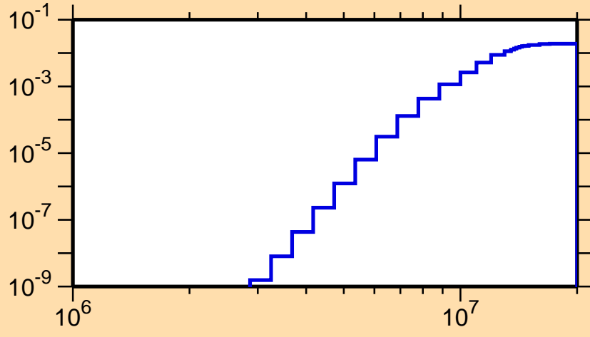
\sigma vs. E for ^{102}\text{Ag}(n,p\alpha)
