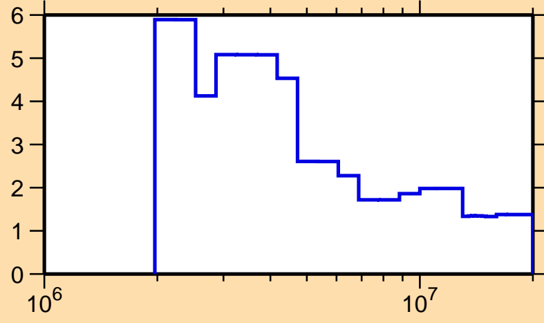
\Delta\sigma/\sigma vs. E for ^{102}\text{Ag}(n, n_{\text{nonel}})
