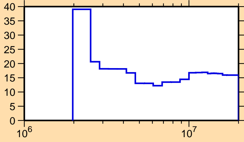
\Delta\sigma/\sigma vs. E for ^{102}\text{Ag}(n,n\text{cont.})
