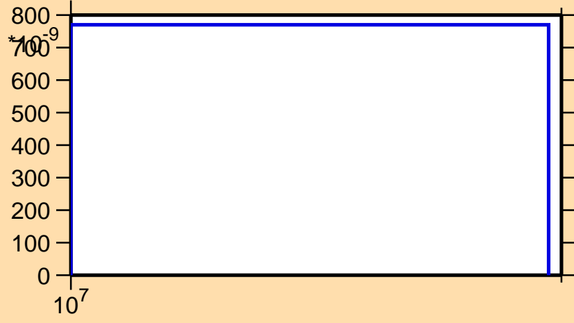
\sigma vs. E for ^{102}\text{Ag} (mt 45)
