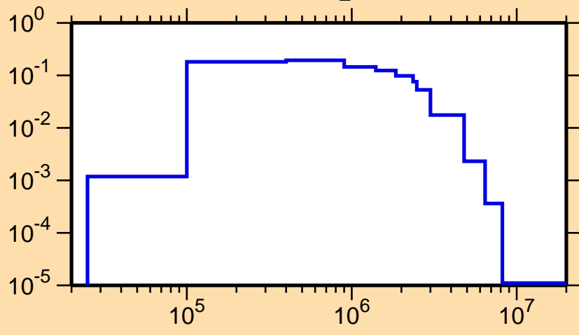
\sigma vs. E for ^{102}\text{Ag}(n,n_2)
