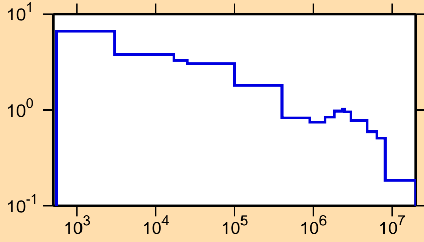
\sigma vs. E for ^{102}\text{Ag}(n,p)
