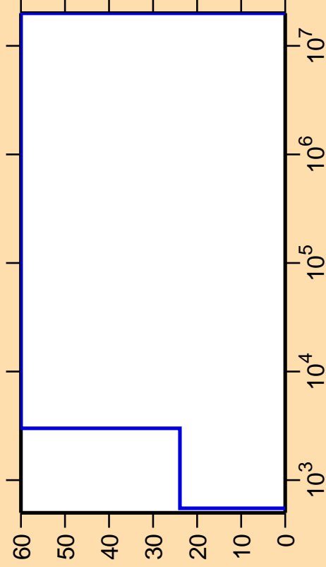
\Delta\sigma/\sigma vs. E for ^{102}\text{Ag}(n,\alpha)
