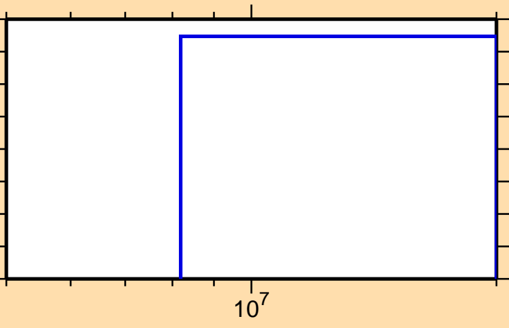
\sigma vs. E for ^{102}\text{Ag}(n,2n\alpha)
