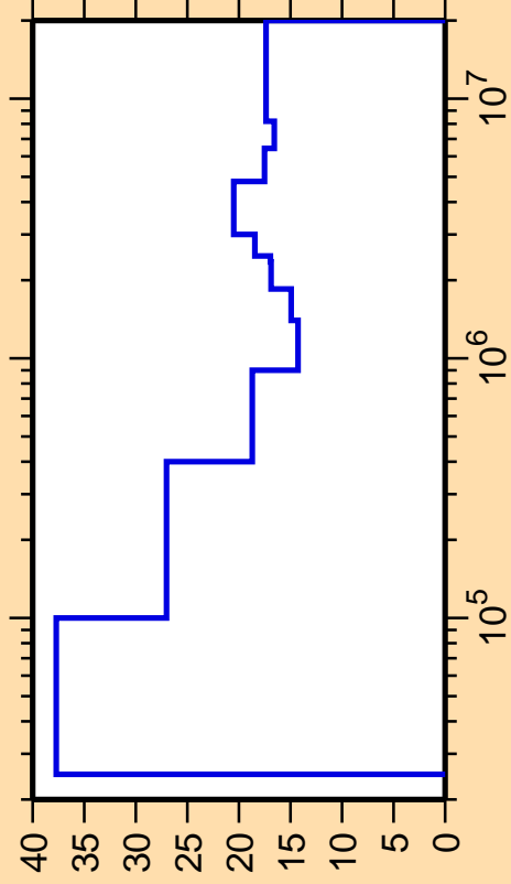
\Delta\sigma/\sigma vs. E for ^{102}\text{Ag}(n,n_2)
