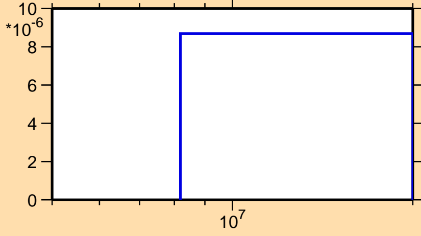
\sigma vs. E for ^{102}\text{Ag}(n,\text{He}3)
