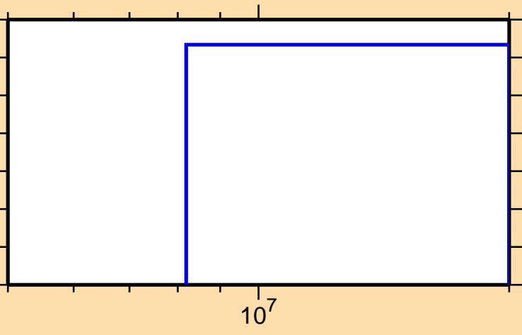
\sigma vs. E for ^{102}\text{Ag}(n,\text{pd})
