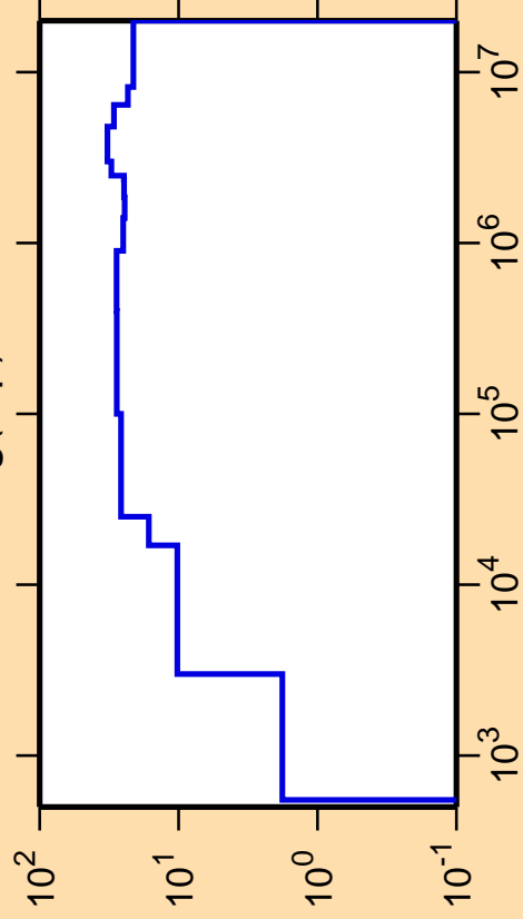
\Delta\sigma/\sigma vs. E for ^{102}\text{Ag}(n,p)
