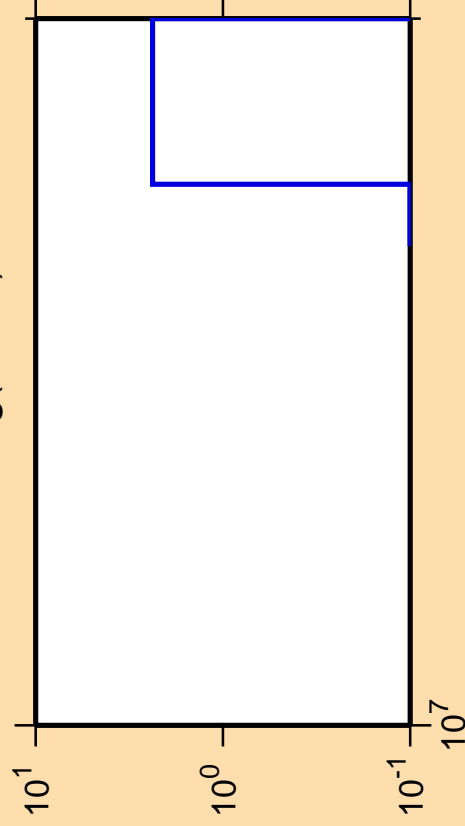
\Delta\sigma/\sigma vs. E for ^{103}\text{Ag}(\text{mt } 34)
