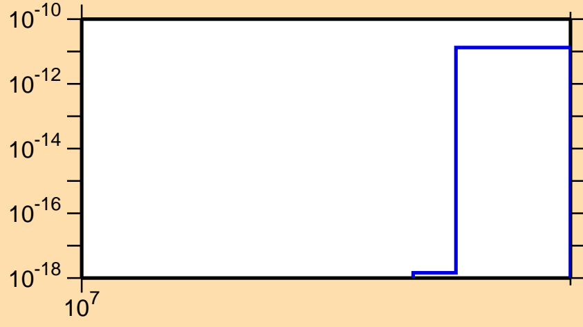
\sigma vs. E for ^{103}\text{Ag}(n,\text{pt})
