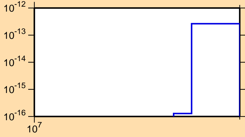
\sigma vs. E for ^{103}\text{Ag}(\text{mt } 34)
