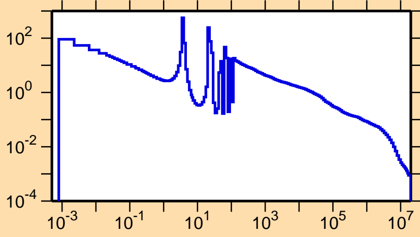
\sigma vs. E for ^{103}\text{Ag}(n,\gamma)
