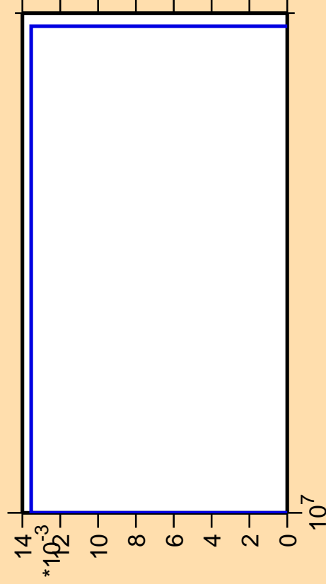
\Delta\sigma/\sigma vs. E for ^{103}\text{Ag} (mt 34)
