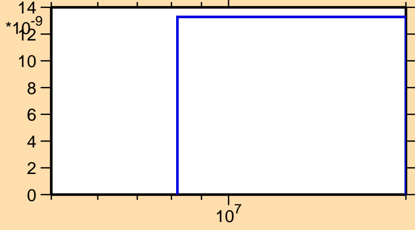
\sigma vs. E for ^{103}\text{Ag}(n,3n)
