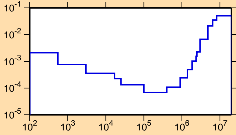
\sigma vs. E for ^{103}\text{Ag}(n,\alpha)
