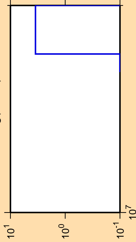
\Delta\sigma/\sigma vs. E for ^{103}\text{Ag} (mt 34)
