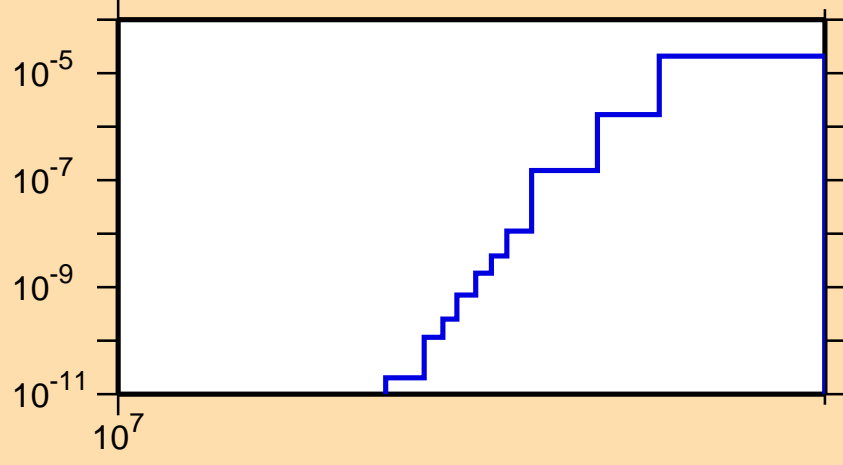
\sigma vs. E for ^{103}\text{Ag}(\text{mt } 45)
