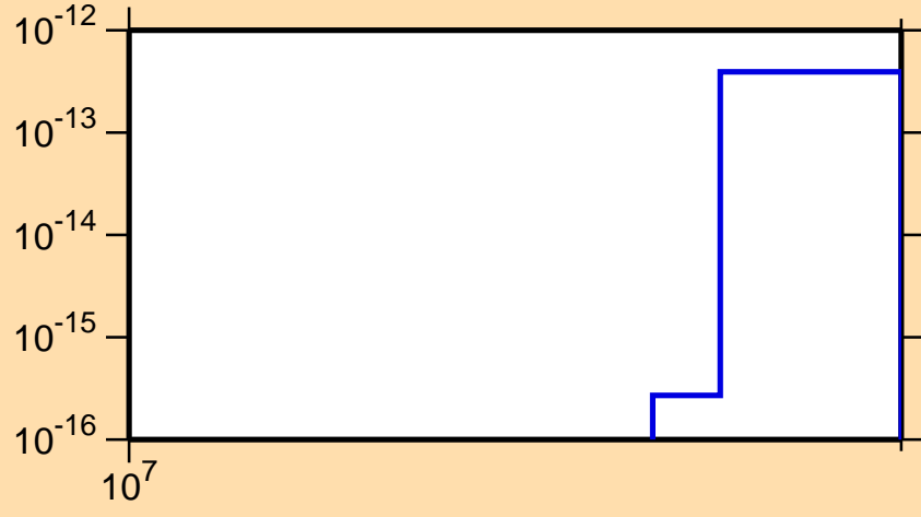
\sigma vs. E for ^{103}\text{Ag} (mt 34)
