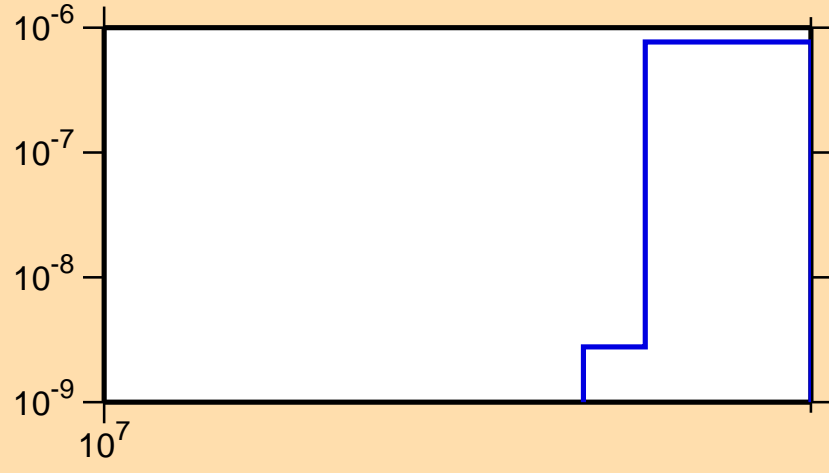
\sigma vs. E for ^{103}\text{Ag}(n,2n\alpha)
