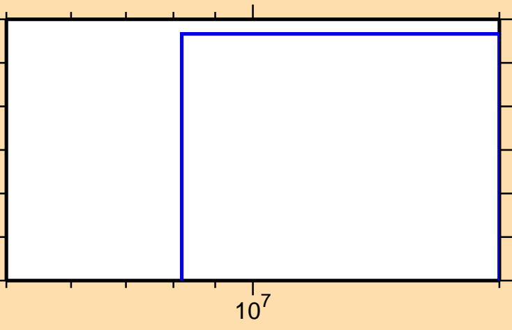
\sigma vs. E for ^{103}\text{Ag}(n,2np)
