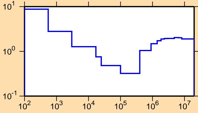
\sigma vs. E for ^{103}\text{Ag}(n,\text{nonel.})
