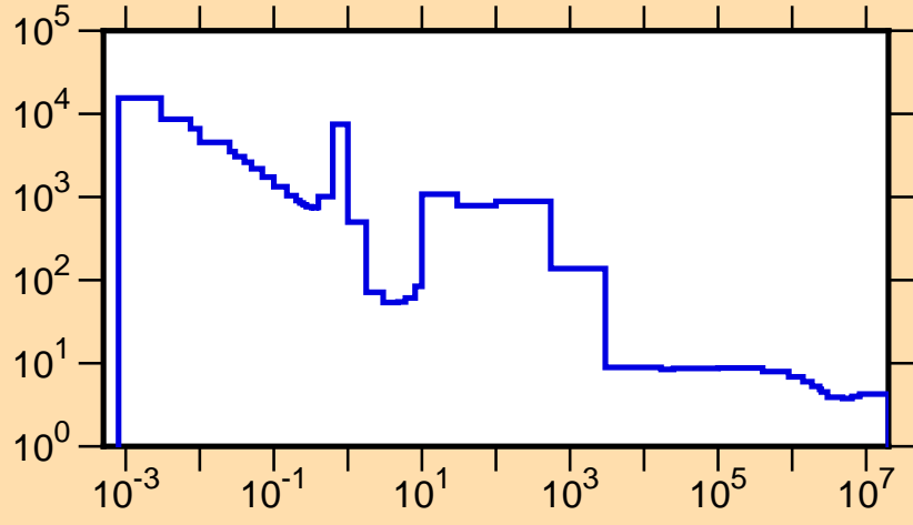
\sigma vs. E for ^{104}\text{Ag}(n,\text{tot.})
