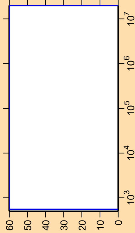
\Delta\sigma/\sigma vs. E for ^{104}\text{Ag}(n,\alpha)
