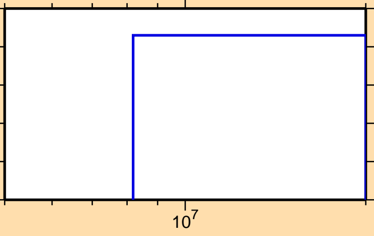
\sigma vs. E for ^{104}\text{Ag}(n,\text{He}3)
