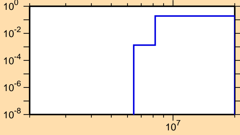
\sigma vs. E for ^{104}\text{Ag}(n,np)
