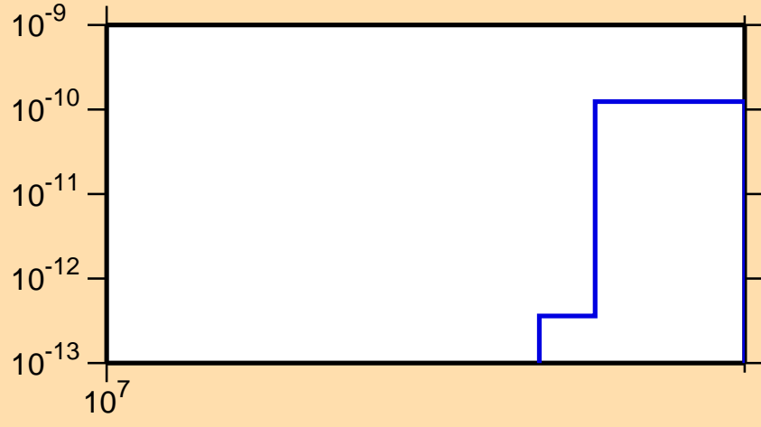
\sigma vs. E for ^{105}\text{Ag}(n,\text{pd})
