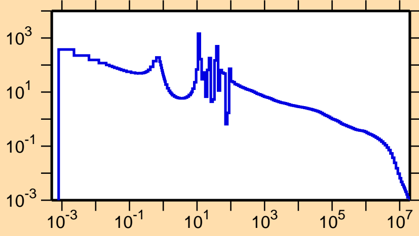
\sigma vs. E for ^{105}\text{Ag}(n,\gamma)
