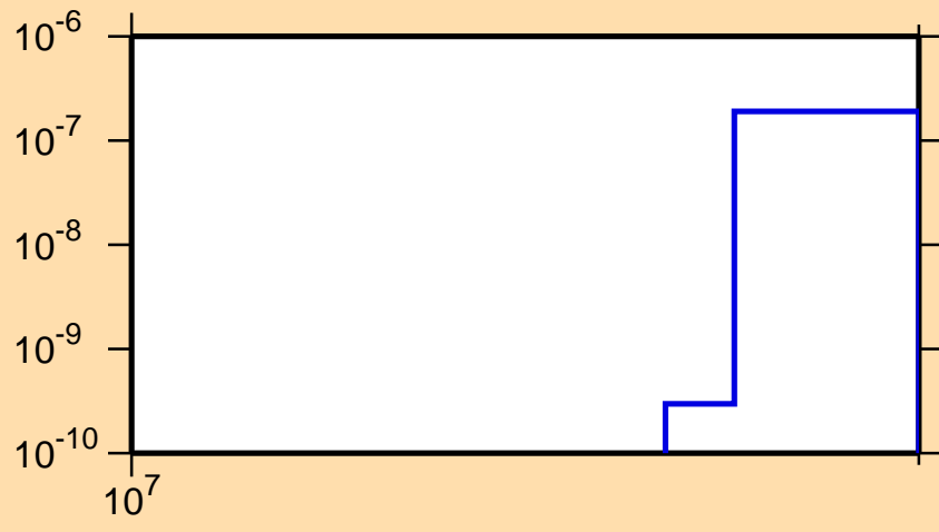
\sigma vs. E for ^{105}\text{Ag}(n,2n\alpha)
