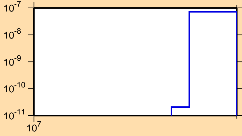
\sigma vs. E for ^{105}\text{Ag}(n,nt)
