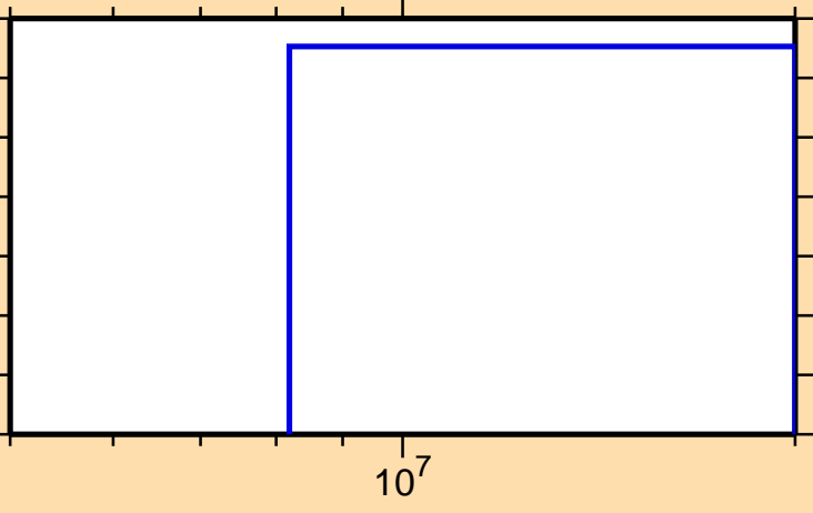
\sigma vs. E for ^{106}\text{Ag}(n,\text{pt})
