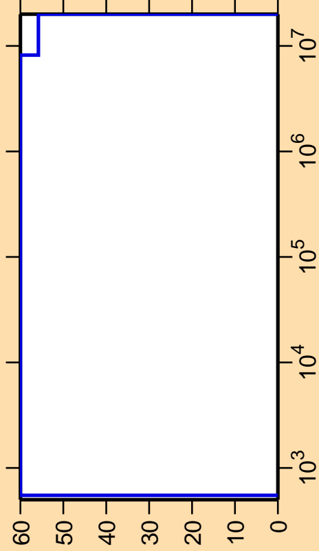
\Delta\sigma/\sigma vs. E for ^{106}\text{Ag}(n,\alpha)
