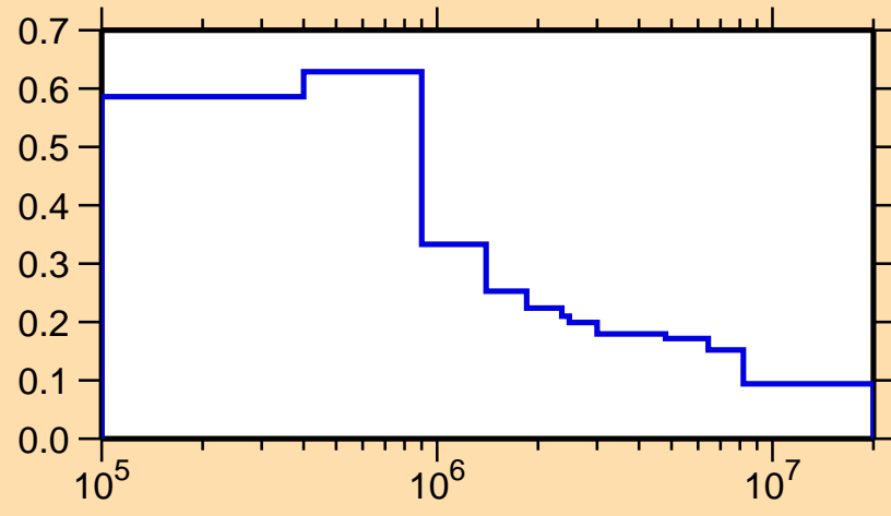
\sigma vs. E for ^{106}\text{Ag}(n,n_2)
