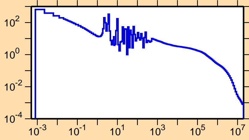
\sigma vs. E for ^{106}\text{Ag}(n,\gamma)
