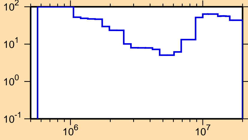
\Delta\sigma/\sigma vs. E for ^{106}\text{Ag}(n,n\text{cont.})
