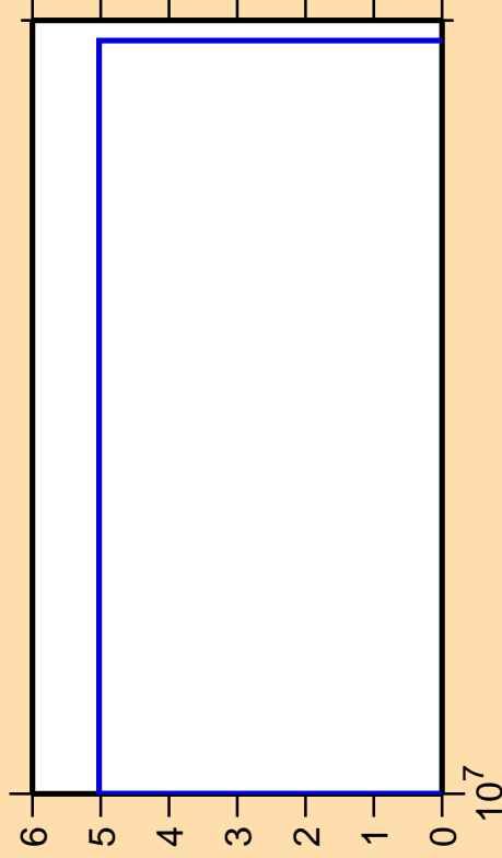
\Delta\sigma/\sigma vs. E for ^{106}\text{Ag}(\text{mt117})
