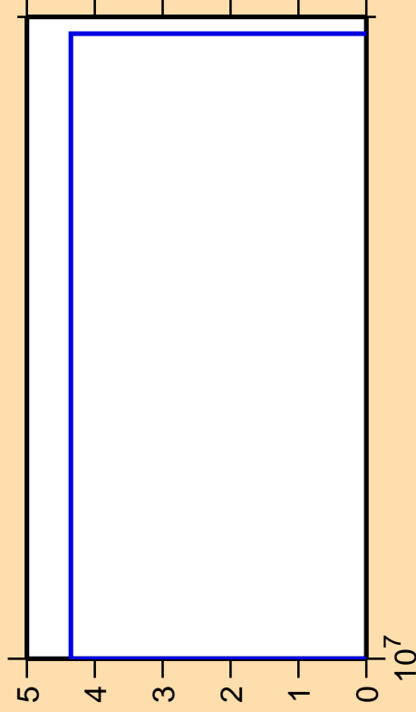
\Delta\sigma/\sigma vs. E for ^{106}\text{Ag}(\text{mt } 45)
