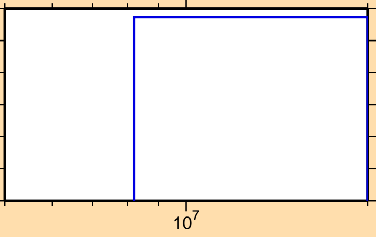
\sigma vs. E for ^{106}\text{Ag}(n,2n\alpha)
