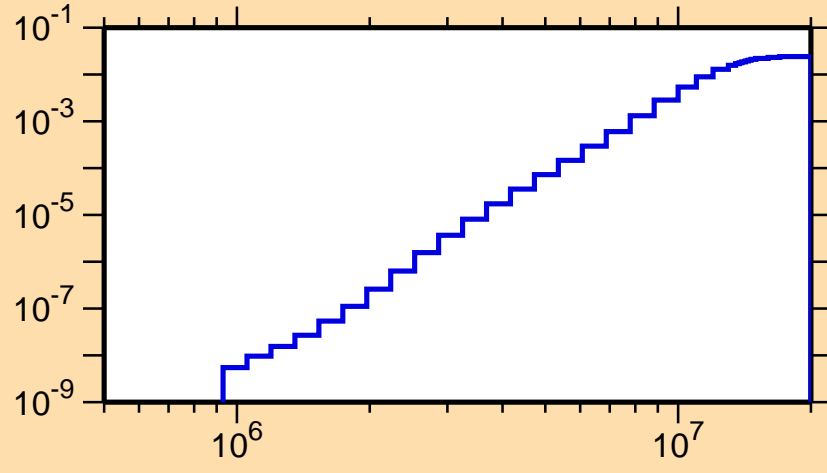
\sigma vs. E for ^{107}\text{Ag}(n,\alpha)
