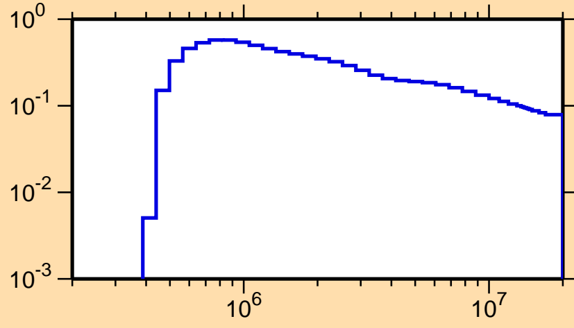
\sigma vs. E for ^{107}\text{Ag}(n,n_4)
