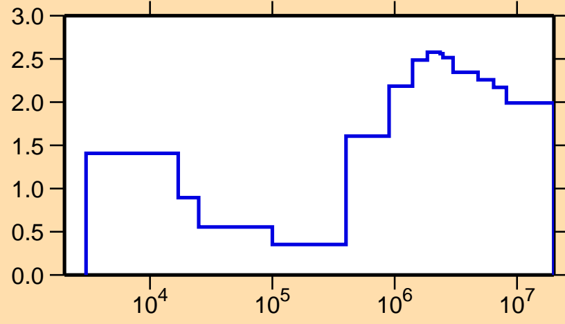
\sigma vs. E for ^{107}\text{Ag}(n,\text{nonel.})
