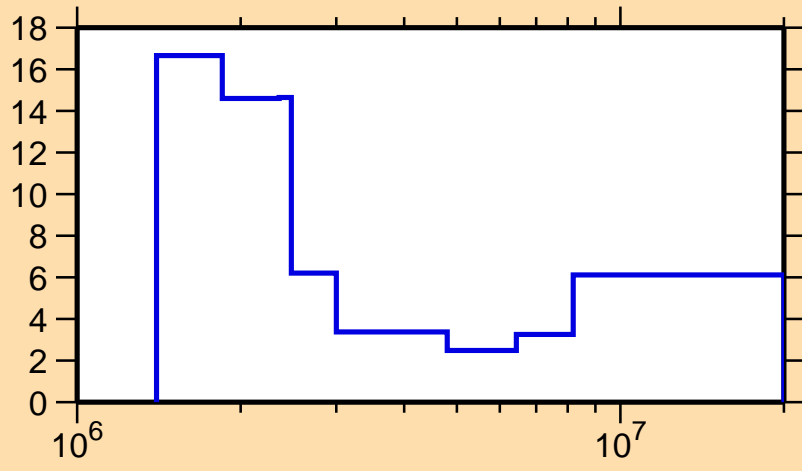
\Delta\sigma/\sigma vs. E for ^{107}\text{Ag}(n, tot.)
