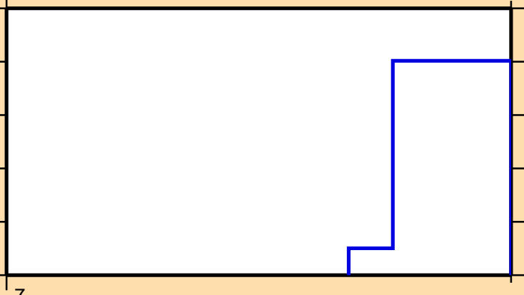
\sigma vs. E for ^{107}\text{Ag}(n,nt)
