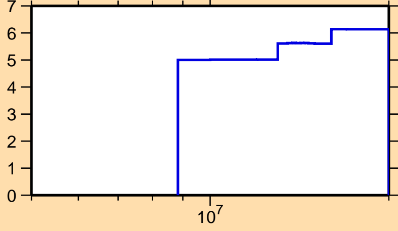
\Delta\sigma/\sigma vs. E for ^{107}\text{Ag}(n,\text{nonel.})
