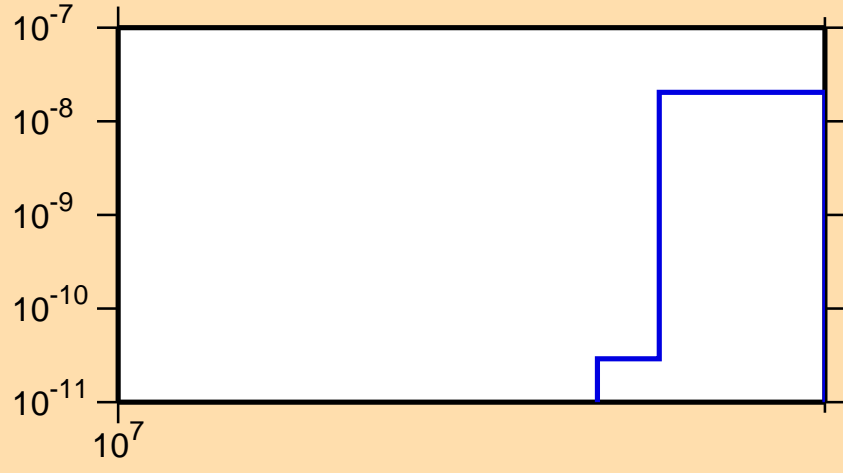
\sigma vs. E for ^{107}\text{Ag}(n,2n\alpha)
