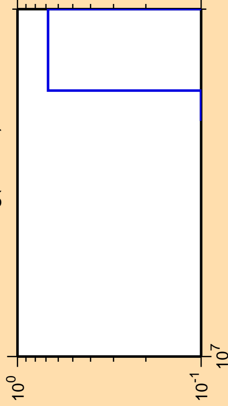
\Delta\sigma/\sigma vs. E for ^{108}\text{Ag}(\text{mt117})
