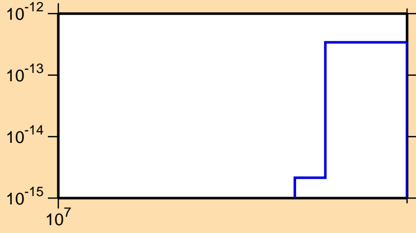
\sigma vs. E for ^{108}\text{Ag}(\text{mt117})
