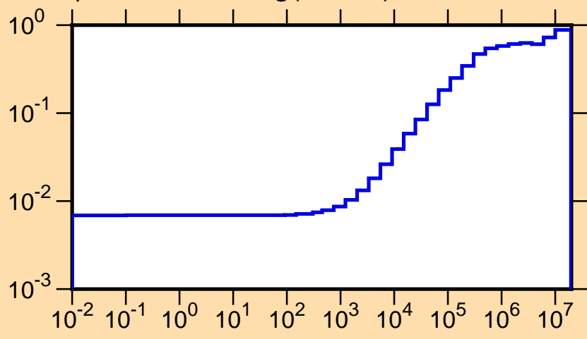
\mu vs. E for ^{108}\text{Ag}(\text{mt251})
