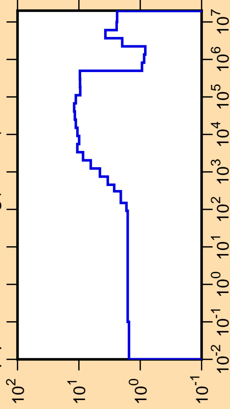
\Delta\mu/\mu vs. E for ^{108}\text{Ag}(\text{mt251})
