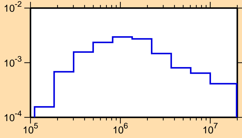
\sigma vs. E for ^{108}\text{Ag}(n,n_2)
