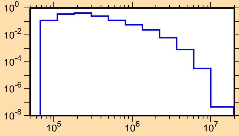
\sigma vs. E for ^{108}\text{Ag}(n,n_1)
