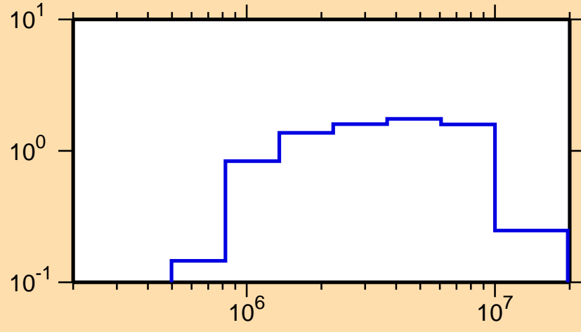
\sigma vs. E for ^{108}\text{Ag}(n,n\text{cont.})
