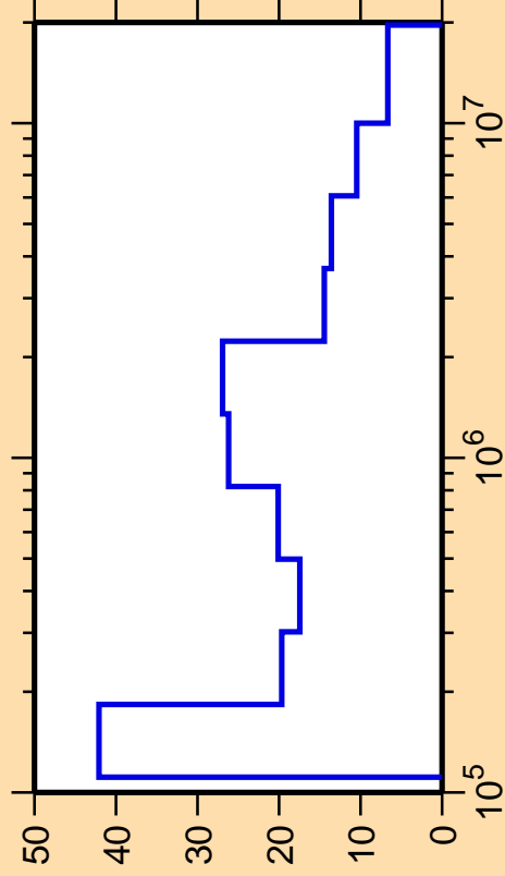
\Delta\sigma/\sigma vs. E for ^{108}\text{Ag}(n,n_2)
