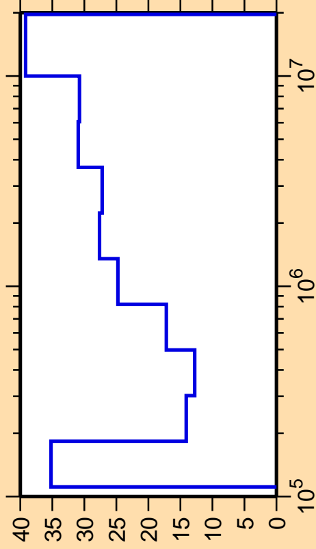
\Delta\sigma/\sigma vs. E for ^{108}\text{Ag}(n,n_3)
