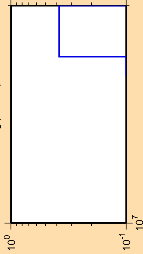
\Delta\sigma/\sigma vs. E for ^{108}\text{Ag}(\text{mt } 45)
