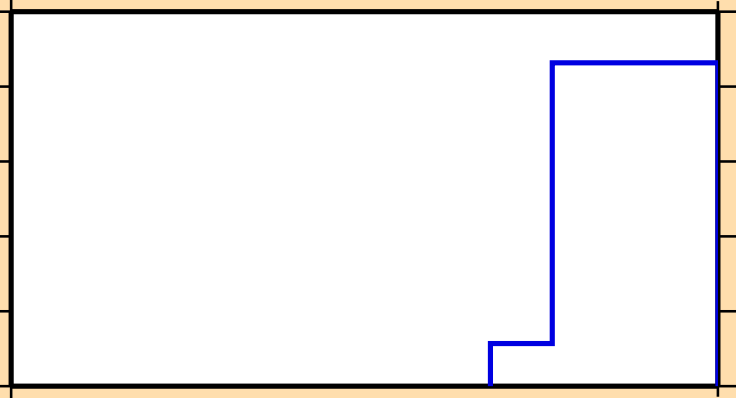
\sigma vs. E for ^{108}\text{Ag}(n,nt)
