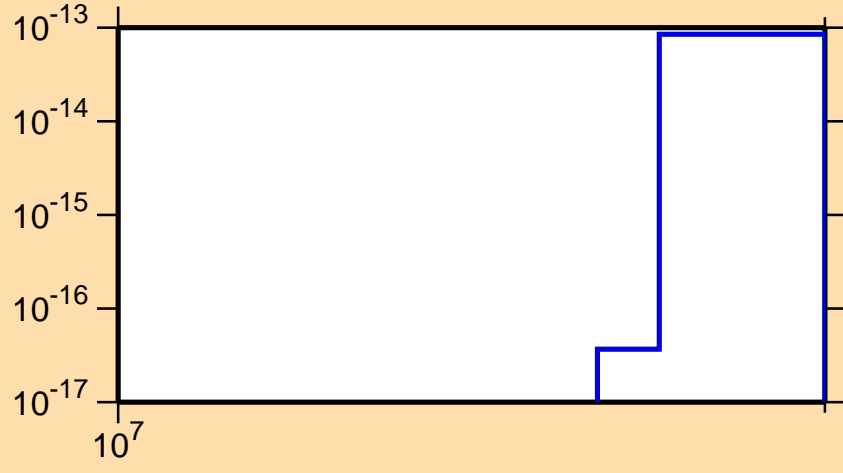
\sigma vs. E for ^{108}\text{Ag}(\text{mt } 45)
