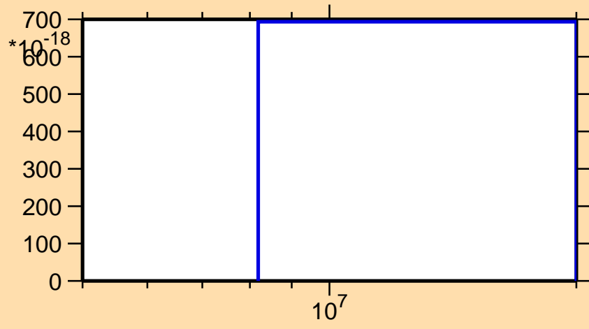
\sigma vs. E for ^{108}\text{Ag}(\text{mt } 45)
