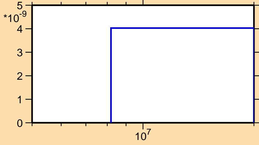
\sigma vs. E for ^{108}\text{Ag}(n,p\alpha)
