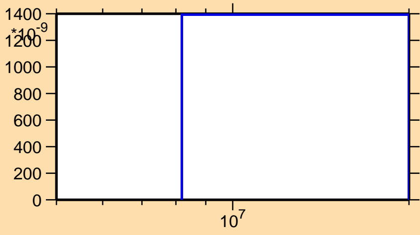
\sigma vs. E for ^{108}\text{Ag}(n,\text{nd})
