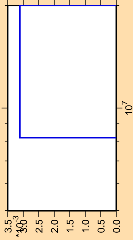
\Delta\sigma/\sigma vs. E for ^{108}\text{Ag}(\text{mt } 45)
