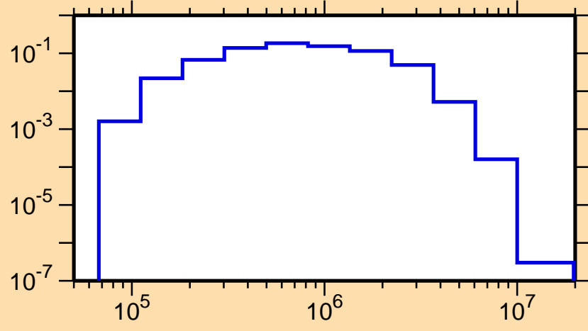
\sigma vs. E for ^{109}\text{Ag}(n,n_1)
