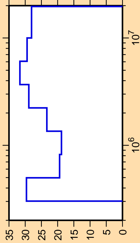
\Delta\sigma/\sigma vs. E for ^{109}\text{Ag}(n,n_4)
