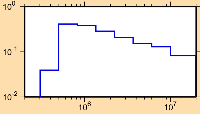
\sigma vs. E for ^{109}\text{Ag}(n,n_4)
