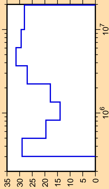
\Delta\sigma/\sigma vs. E for ^{109}\text{Ag}(n,n_3)
