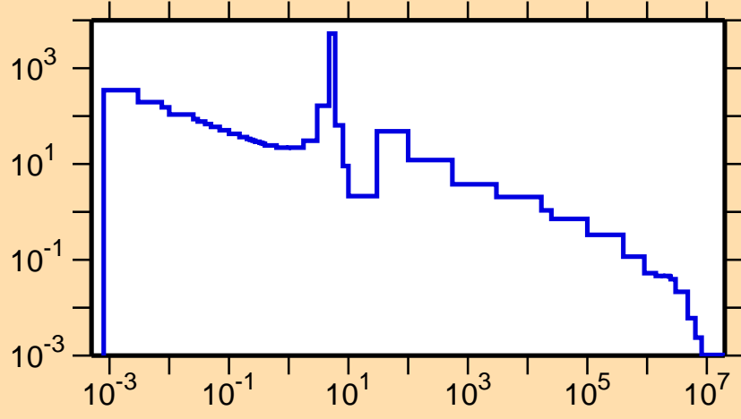
\sigma vs. E for ^{109}\text{Ag}(n,\gamma)
