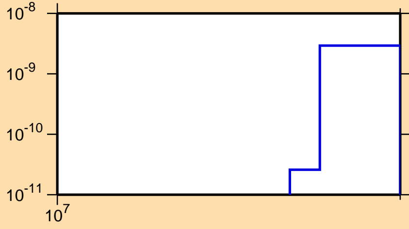
\sigma vs. E for ^{109}\text{Ag}(n,\text{He}3)
