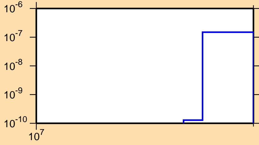
\sigma vs. E for ^{109}\text{Ag}(n,nt)
