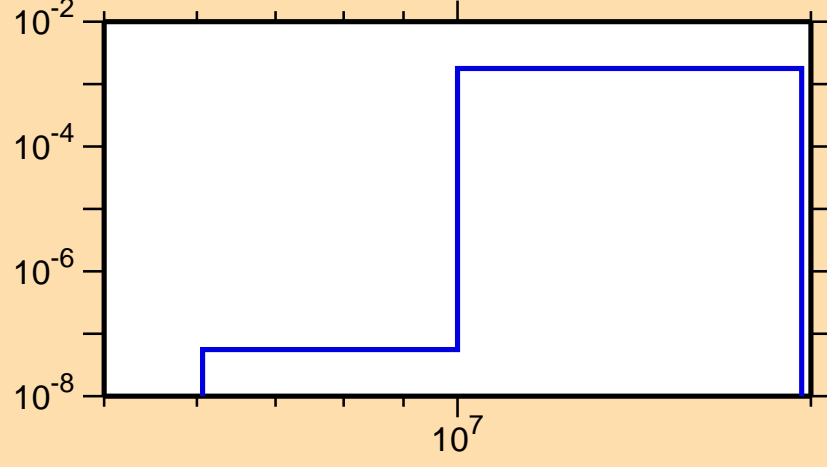
\sigma vs. E for ^{109}\text{Ag}(n,d)
