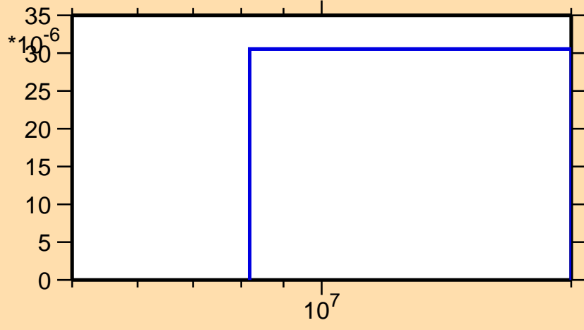
\sigma vs. E for ^{109}\text{Ag}(n,t)
