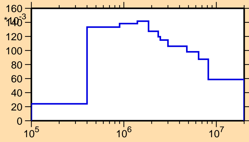
\sigma vs. E for ^{109}\text{Ag}(n,n_3)
